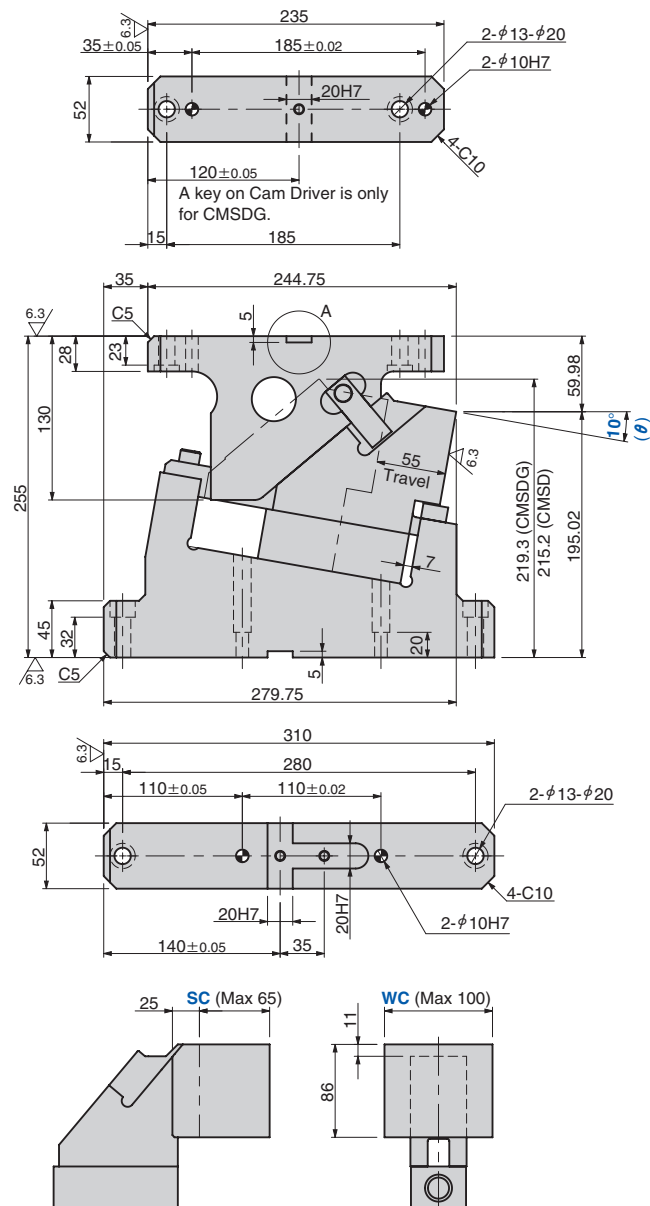
● Cam Diagram
