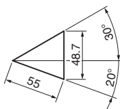
● Cam Diagram
